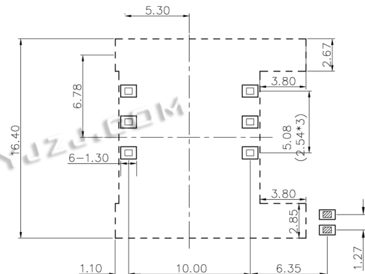
REFERENCE PC BOARD LAYOUT
